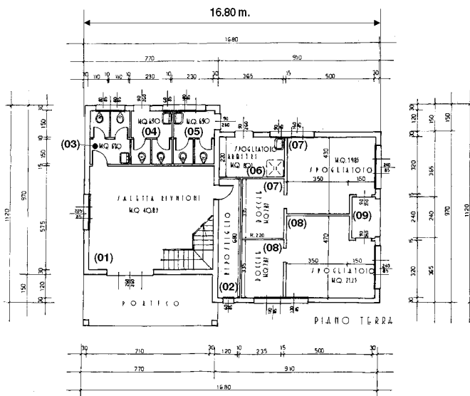
PIANO TERRA (01)
